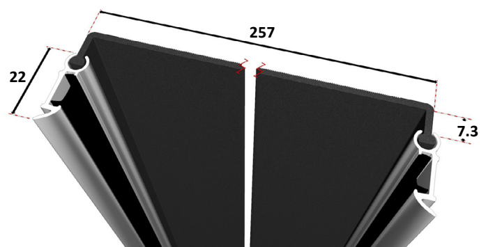
Astro FingerKeeper Industrial TPV Wide Profile (measurements in mm)
