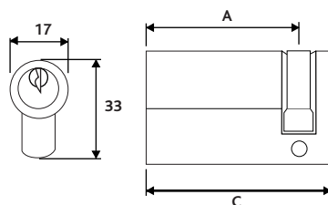
Single Euro Profile Cylinder
